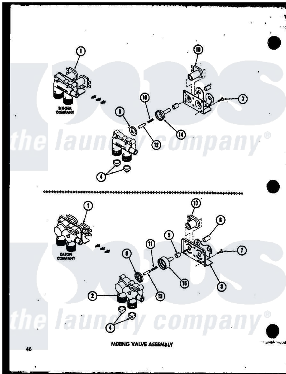
Amana Residential Amana TAA600 (BOM: P7575110W) Washer Parts Parts Diagram 07 - MIXING VALVE ASSY
