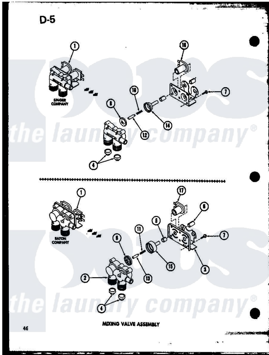
Amana Residential Amana TAA600 (BOM: P7575116W) Washer Parts Parts Diagram 08 - MIXING VALVE ASSY
