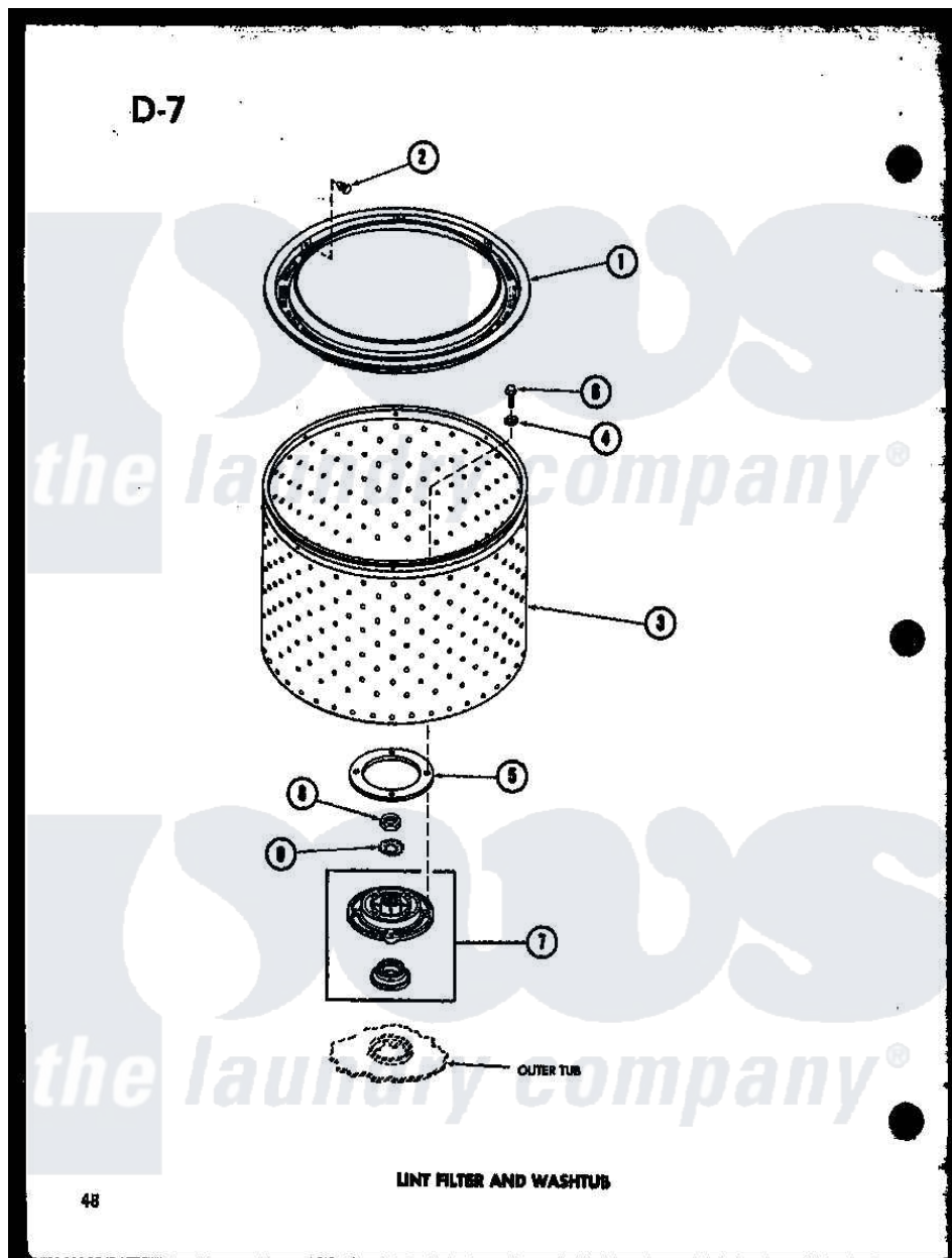
Amana Residential Amana TAA800 (BOM: P7575103W) Washer Parts Parts Diagram 07 - LINT FILTER AND WASHTUB
