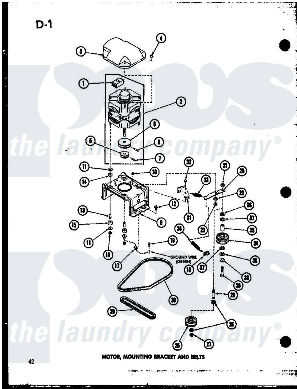
Amana Residential Amana TAA800 (BOM: P7575103W) Washer Parts Parts Diagram 09 - MOTOR Click on the part number to view part
