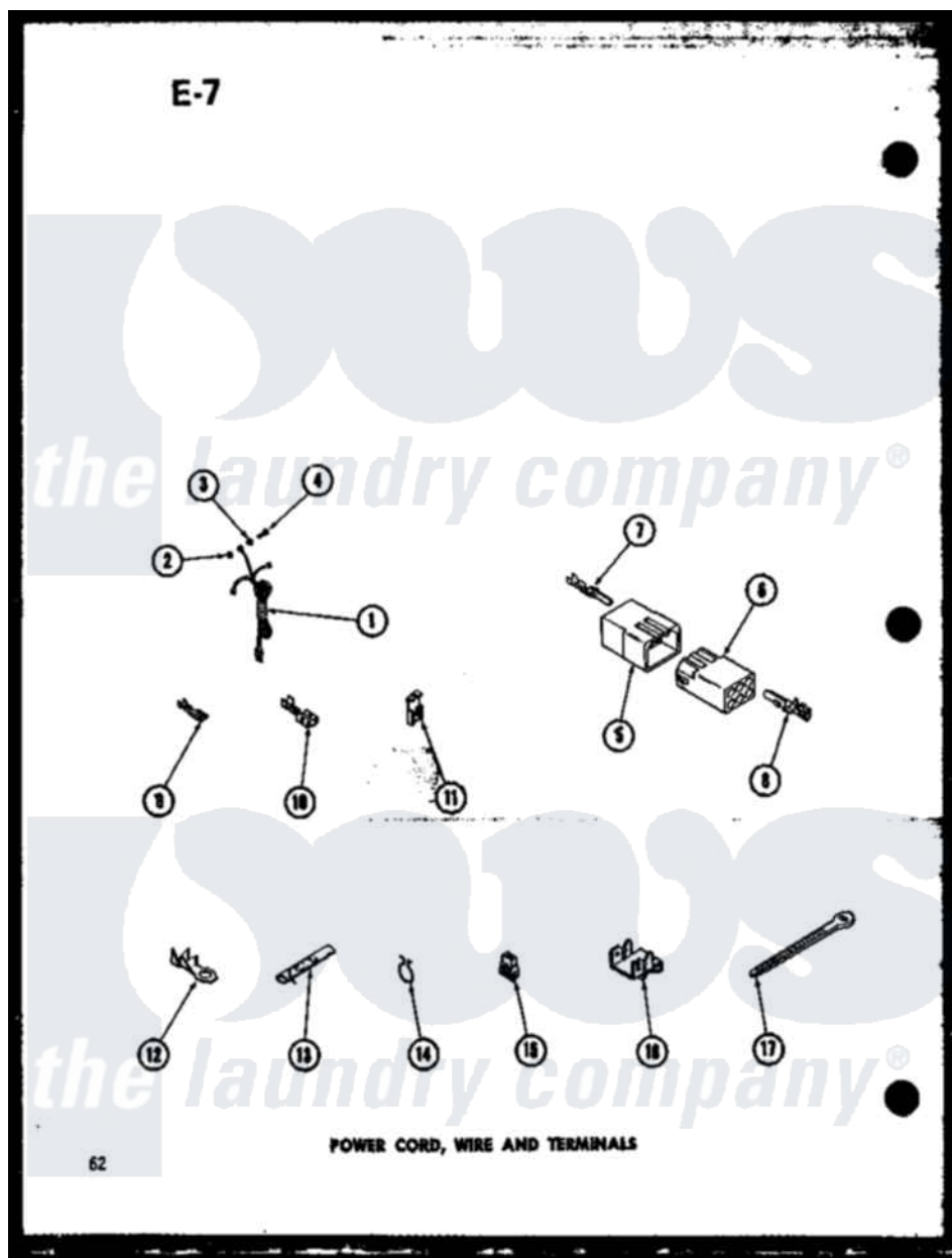
Amana Residential Amana TAA800 (BOM: P7575103W) Washer Parts Parts Diagram 11 - POWER CORD Click on the part number to view part
