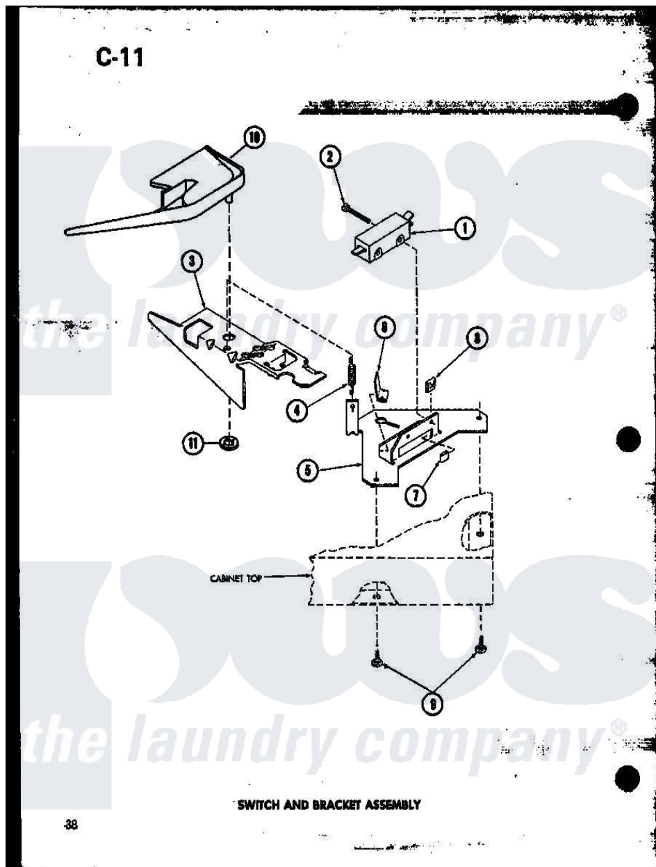
Amana Residential Amana TAA800 (BOM: P7575103W) Washer Parts Parts Diagram 13 - SWITCH AND BRACKET ASSY
