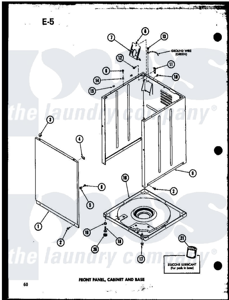
Amana Residential Amana TAA800 (BOM: P7575107W) Washer Parts Parts Diagram 05 - FRONT PANEL Click on the part number to view part
