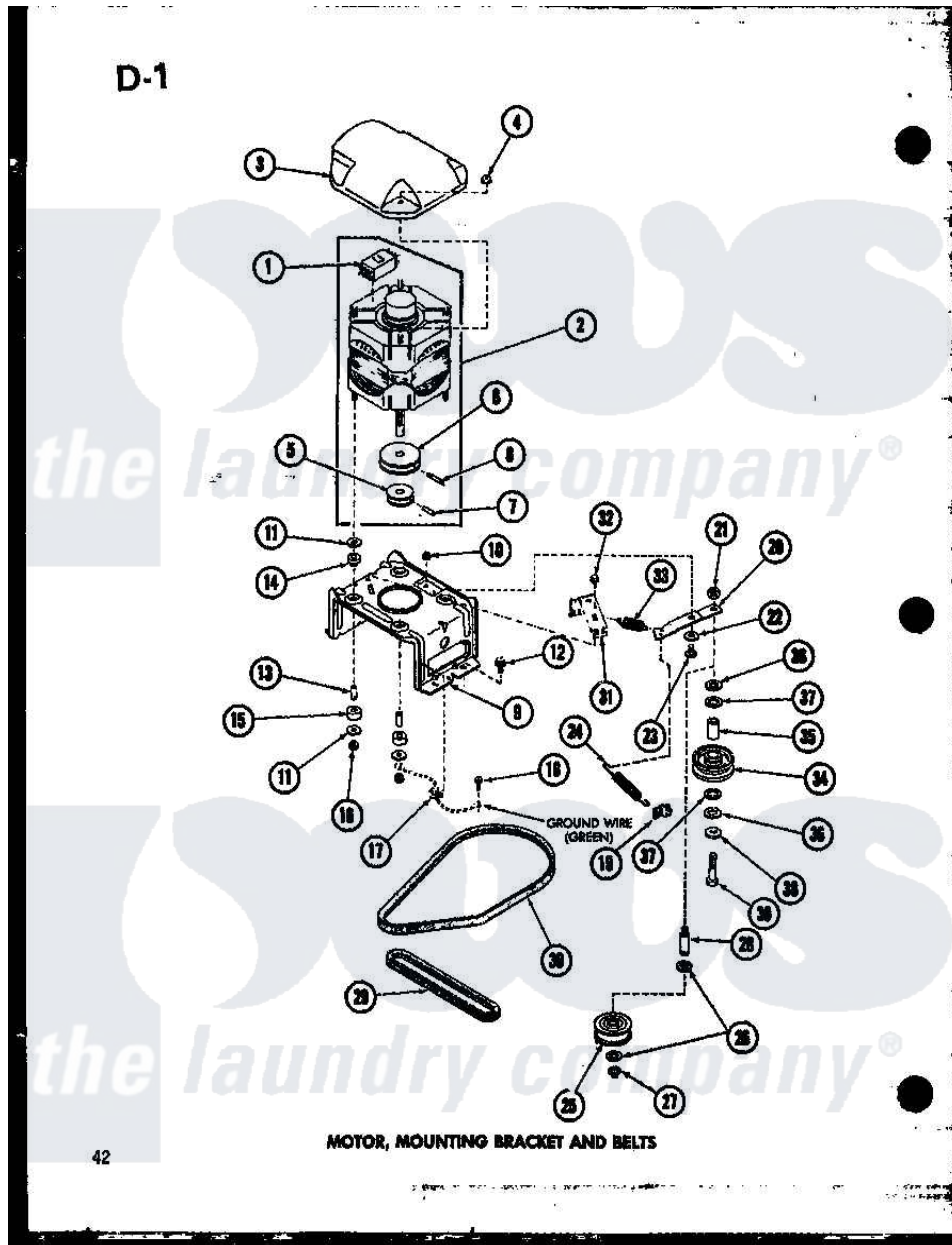
Amana Residential Amana TAA800 (BOM: P7575107W) Washer Parts Parts Diagram 09 - MOTOR Click on the part number to view part
