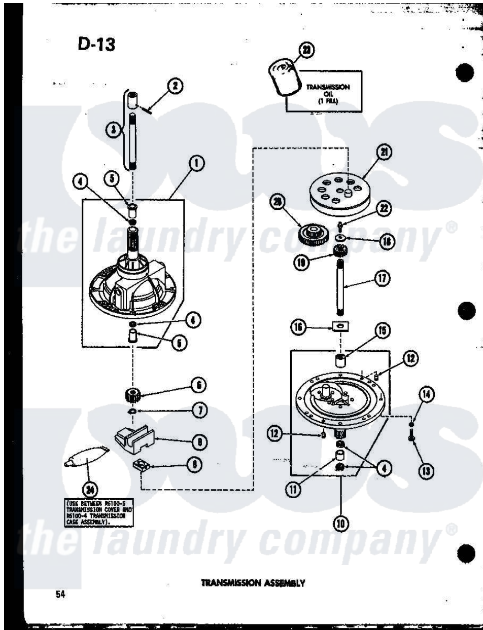
Amana Residential Amana TAA800 (BOM: P7575107W) Washer Parts Parts Diagram 14 - TRANSMISSION ASSY Click on the part number to view part
