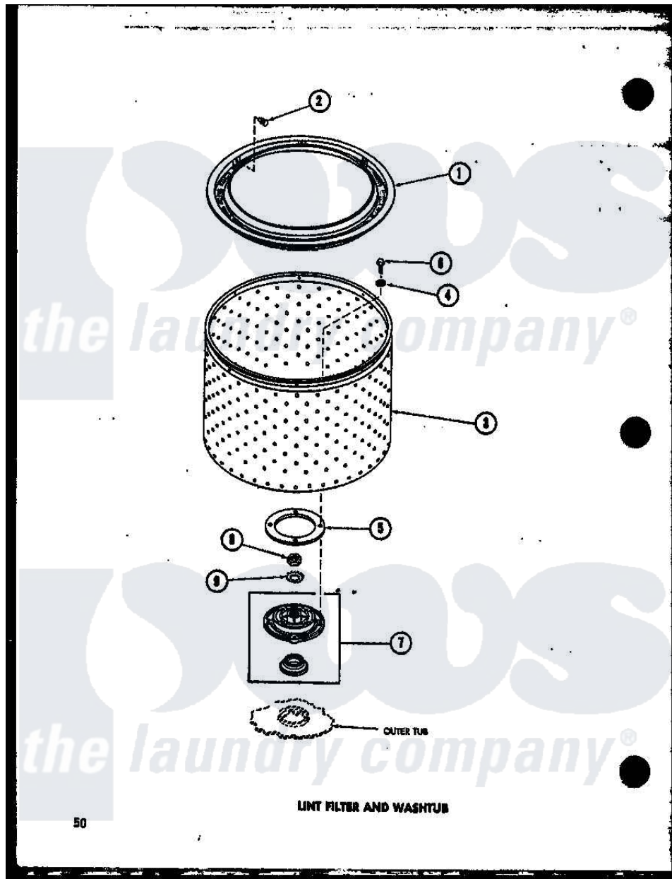
Amana Residential Amana TAA800 (BOM: P7575111W) Washer Parts Parts Diagram 06 - LINT FILTER AND WASHTUB
