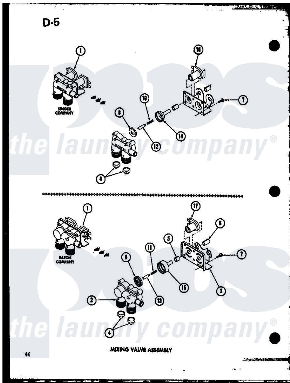
Amana Residential Amana TAA800 (BOM: P7575117W) Washer Parts Parts Diagram 08 - MIXING VALVE ASSY
