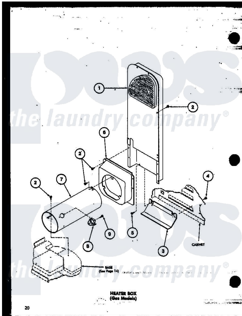
Amana Residential Amana TEA400 (BOM: P7575203W) Dryer Parts Parts Diagram 06 - HEATER BOX Click on the part number to view part
