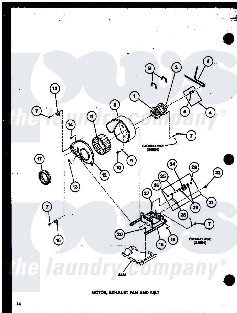
Amana Residential Amana TEA600 (BOM: P7575201W) Dryer Parts Parts Diagram 09 - MOTOR Click on the part number to view part
