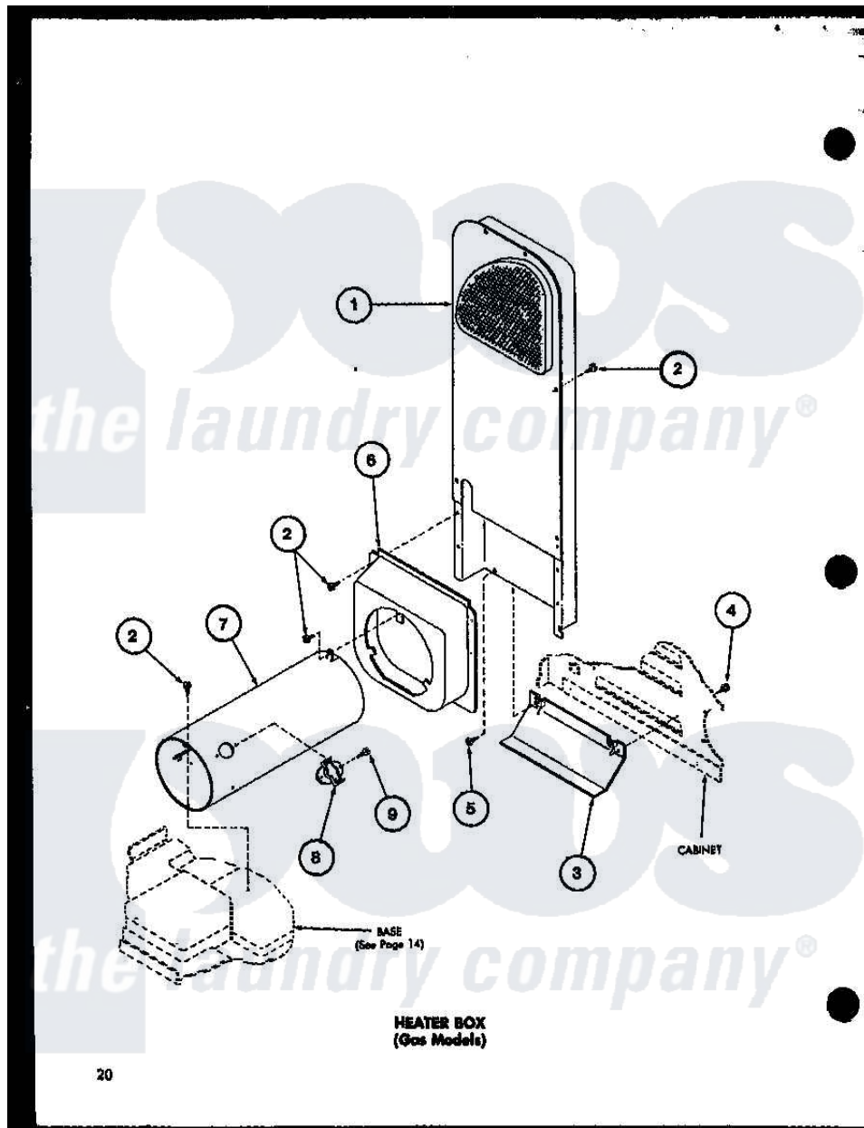
Amana Residential Amana TGA800 (BOM: P7704107W) Dryer Parts Parts Diagram 06 - HEATER MODELS)
