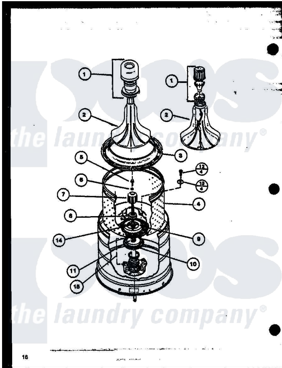
Amana Residential Amana TW3303G (BOM: P1128408W G) Washer Parts Parts Diagram 04 - Page 6 Click on the part number to view part
