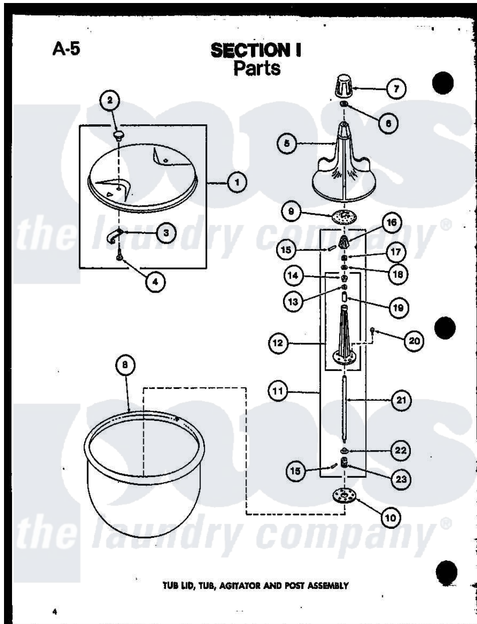
Amana Residential Amana TWA-202 (BOM: P7575302W) Washer Parts Parts Diagram 07 - TUB LID Click on the part number to view part
