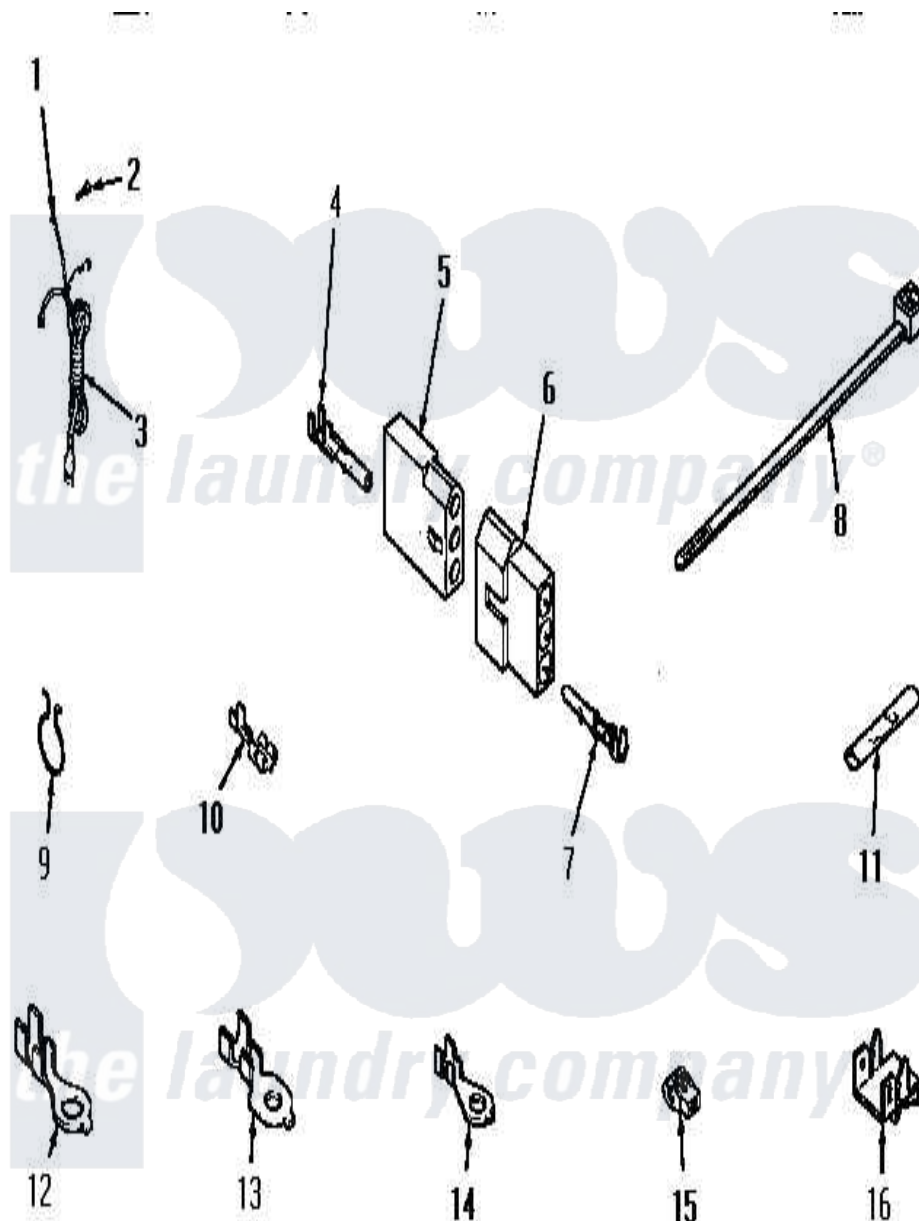
Amana Residential Amana VA6013 Washer Parts Parts Diagram 10 - POWER CORD, WIRE HARNESSSES, WIRE & TERM
