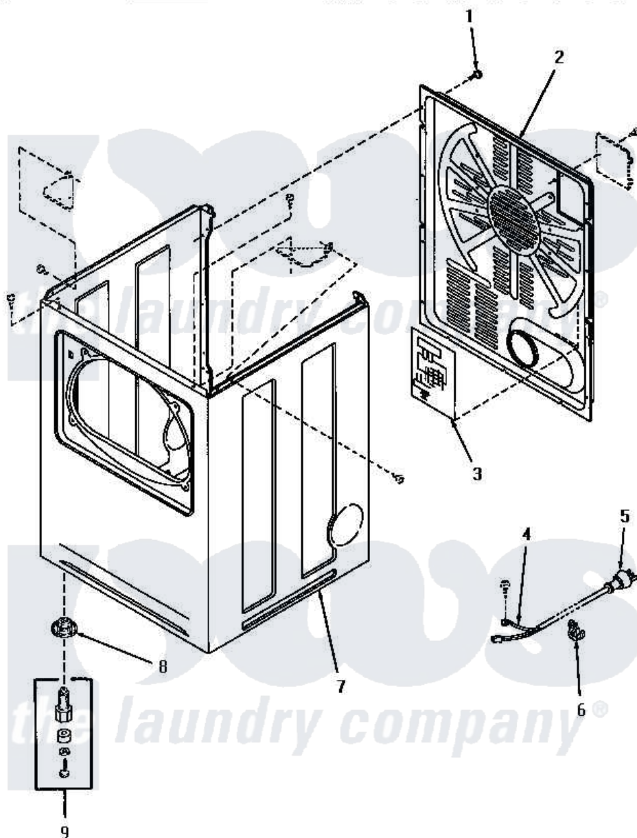
Amana Residential Amana YE1203 Washer Parts Parts Diagram 01 - CABINET ASSY, REAR PANEL AND POWER CORD
