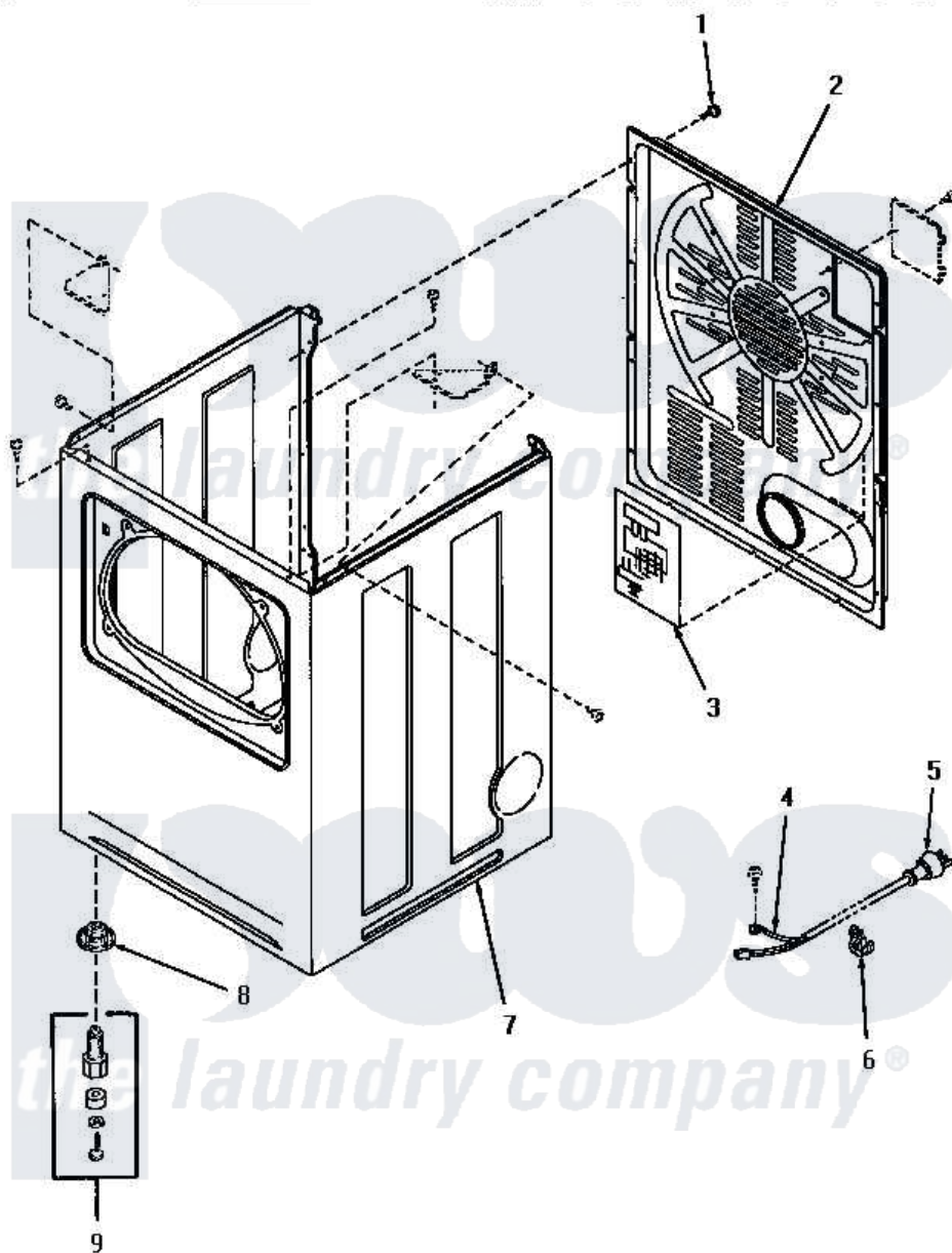
Amana Residential Amana YE1243 Washer Parts Parts Diagram 01 - CABINET ASSY, REAR PANEL AND POWER CORD
