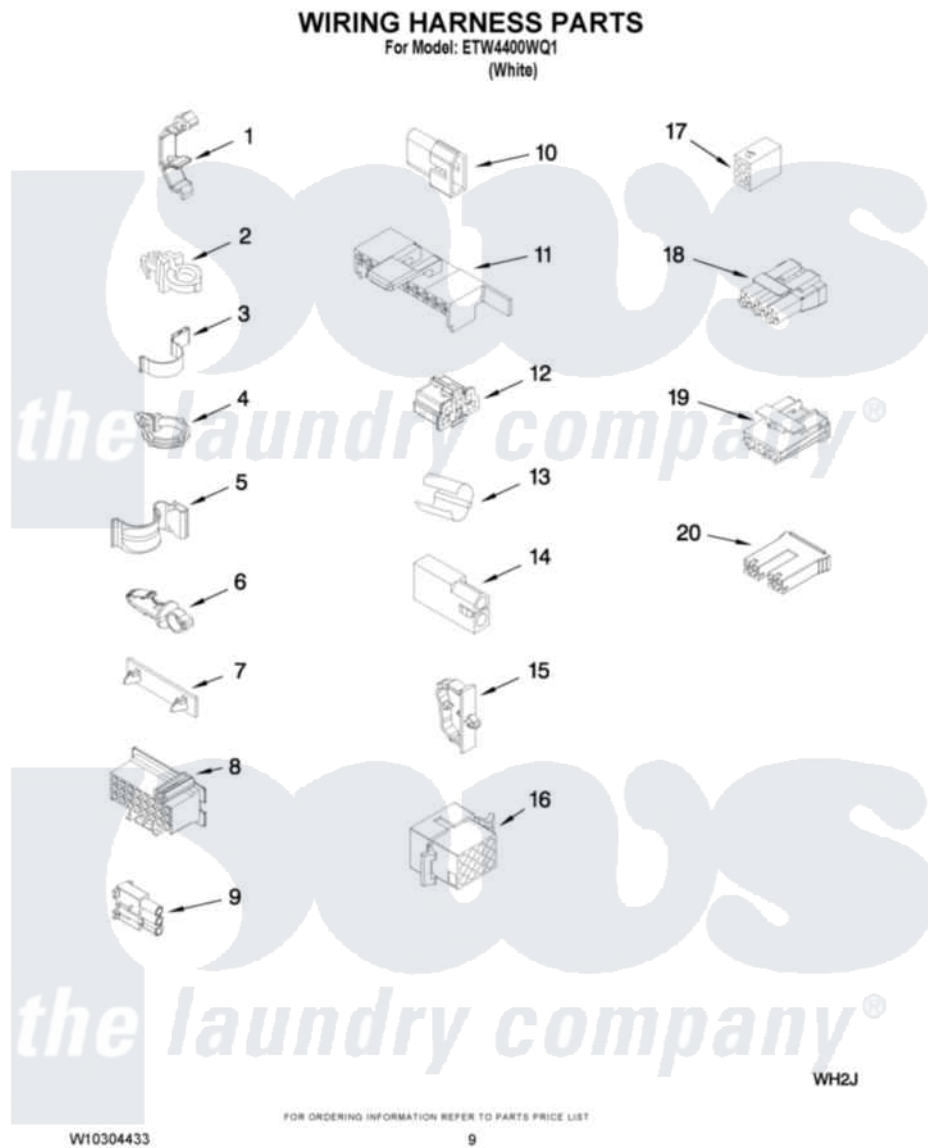
Estate Residential Estate ETW4400WQ1 Washer Parts Parts Diagram 06 - WIRING HARNESS PARTS Click on the part number to view part
