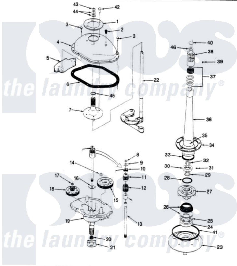
Hoover Residential Hoover A1408 Washer Parts Parts Diagram 08 - TRANSMISSION (REV. E-G) Click on the part number to view part
