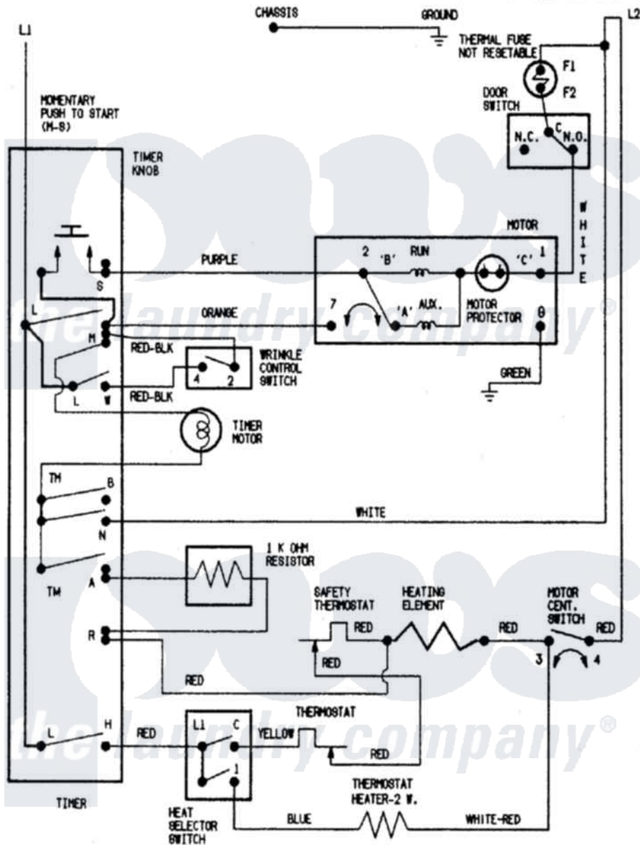
Hoover Residential Hoover HYE2200AKW Dryer Parts Parts Diagram 08 - WIRING INFORMATION Click on the part number to view part
