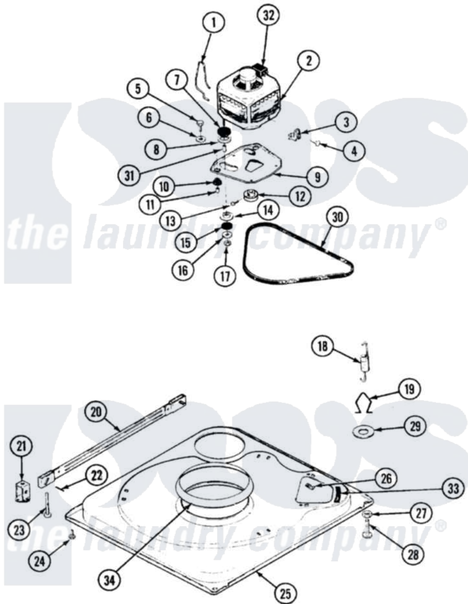
Hoover Residential Hoover SHWA2501A Washer Parts Parts Diagram 01 - BASE Click on the part number to view part
