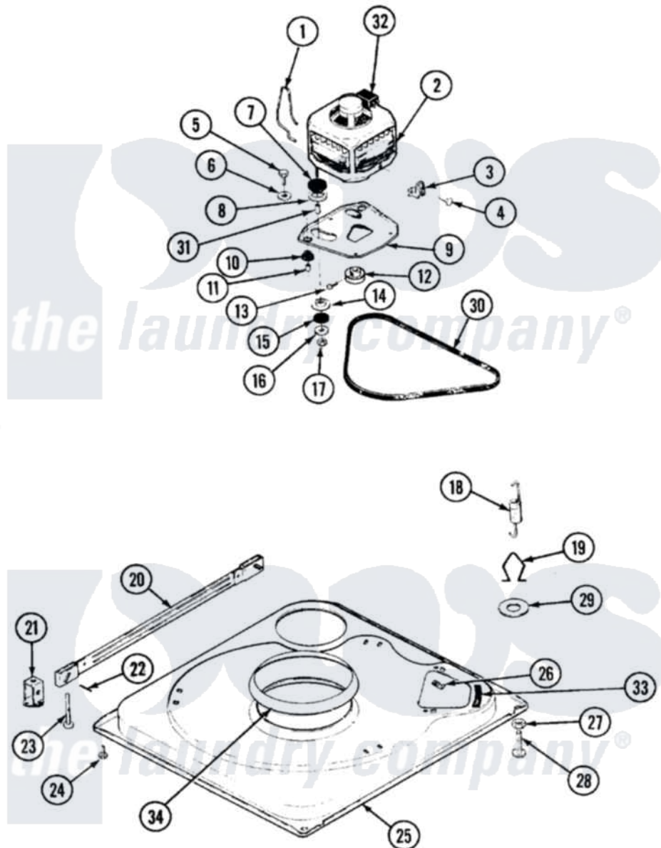
Hoover Residential Hoover SHWA2506WT Washer Parts Parts Diagram 01 - BASE Click on the part number to view part
