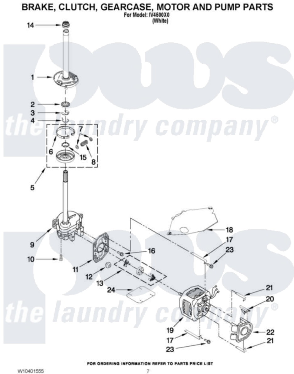
Inglis Residential Inglis IV4500X0 Washer Parts Parts Diagram 04 - BRAKE, CLUTCH, GEARCASE, MOTOR AND PUMP PARTS
