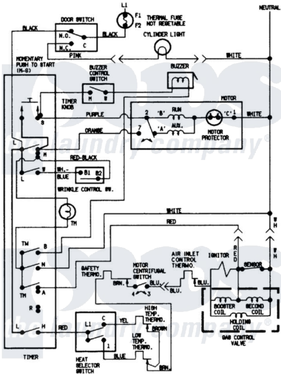
Jenn-Air Residential Jenn-Air JDG1000W Dryer Parts Diagram 07 - WIRING INFORMATION Click on the part number to view part
