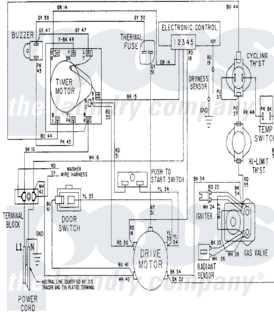
Jenn-Air Residential Jenn-Air LSG2704W Stacked Washer and Dryer Parts Parts Diagram 15 - WIRING INFORMATION-DRYER
