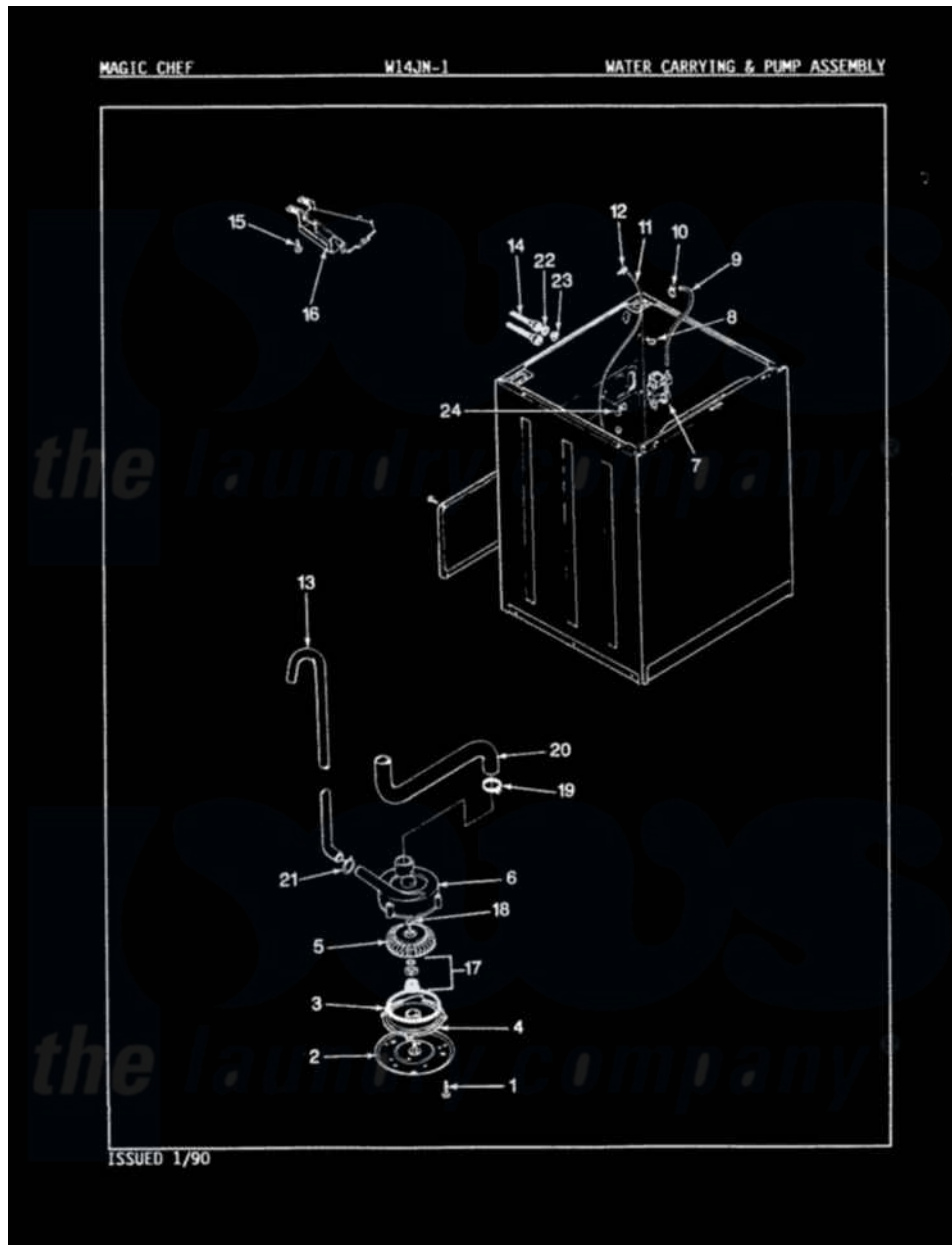
Magic Chef Residential Magic Chef W14JN1 Washer Parts Parts Diagram 17 - WATER CARRYING & PUMP ASSY. (REV. A-D)
