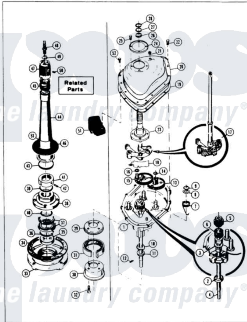
Magic Chef Residential Magic Chef W18FA1 Washer Parts Parts Diagram 03 - TRANSMISSION Click on the part number to view part
