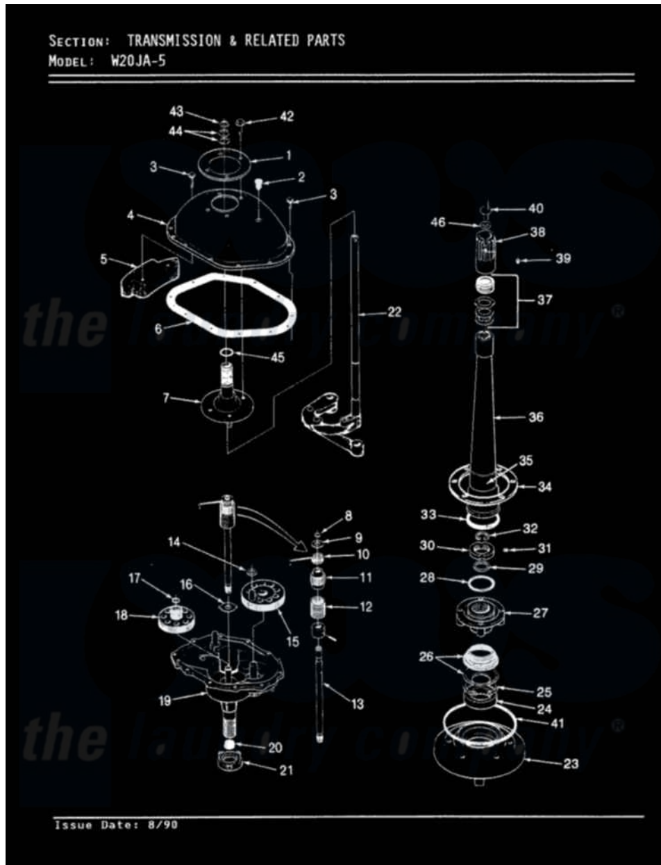
Magic Chef Residential Magic Chef W20JA5 Washer Parts Parts Diagram 08 - TRANSMISSION (W20JA5)(REV. A-D) Click on the part number to view part
