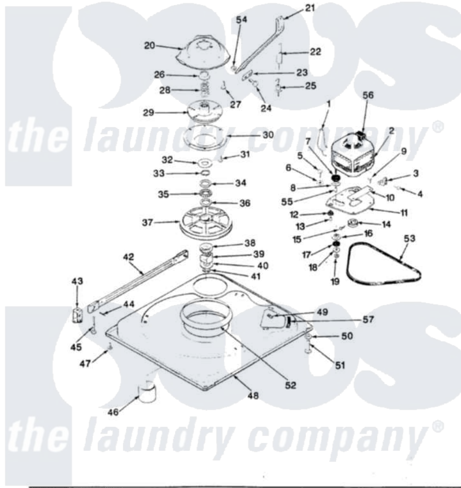
Magic Chef Residential Magic Chef W26HN2K Washer Parts Parts Diagram 01 - BASE & DRIVE (REV. A-D) Click on the part number to view part
