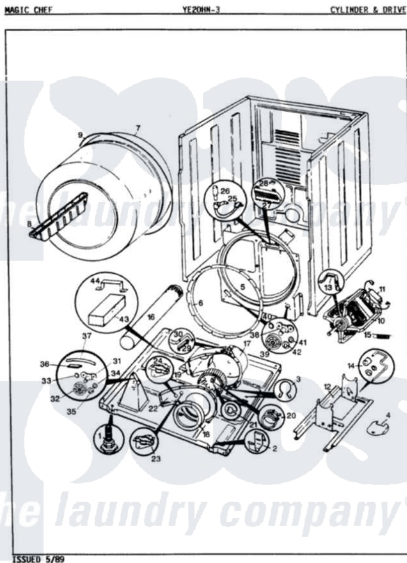
Magic Chef Residential Magic Chef YE20HN3 Dryer Parts Parts Diagram 05 - CYLINDER & DRIVE (REV. A-D) Click on the part number to view part
