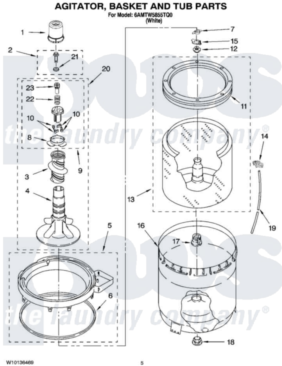
Maytag Residential Maytag 6AMTW5855TQ0 Washer Parts Parts Diagram 03 - AGITATOR, BASKET AND TUB PARTS
