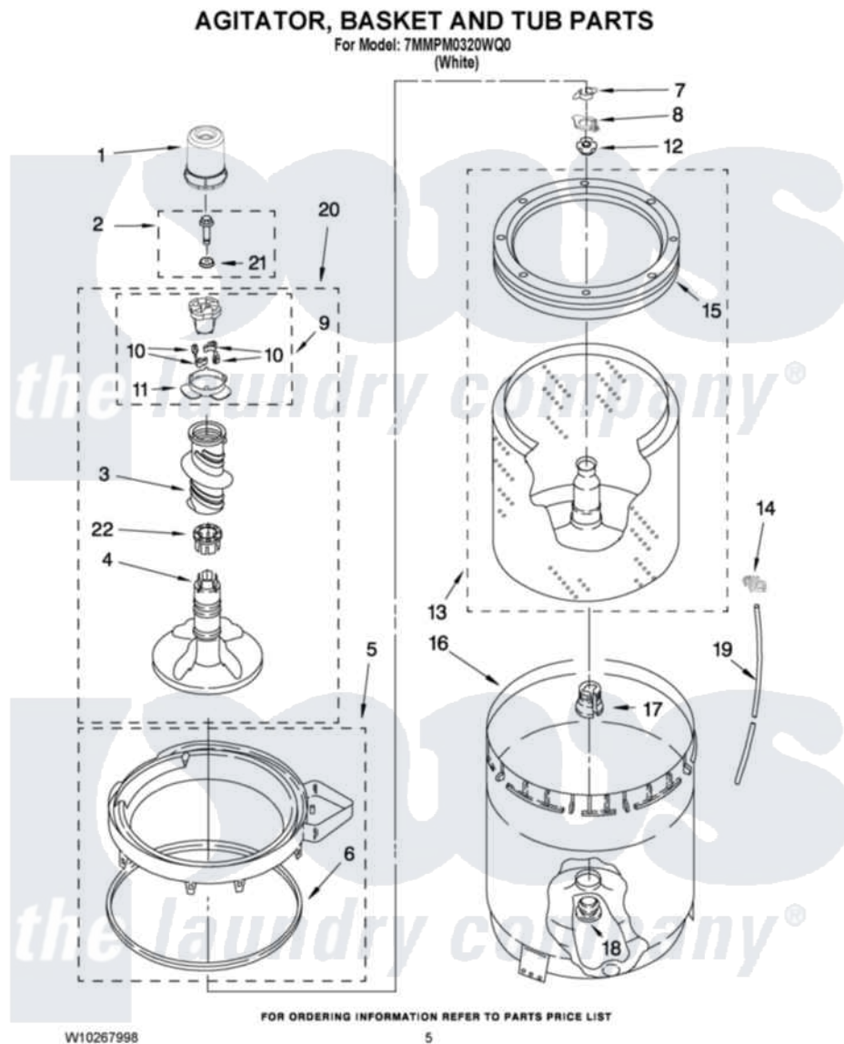
Maytag Residential Maytag 7MMPM0320WQ0 Washer Parts Parts Diagram 03 - AGITATOR, BASKET AND TUB PARTS
