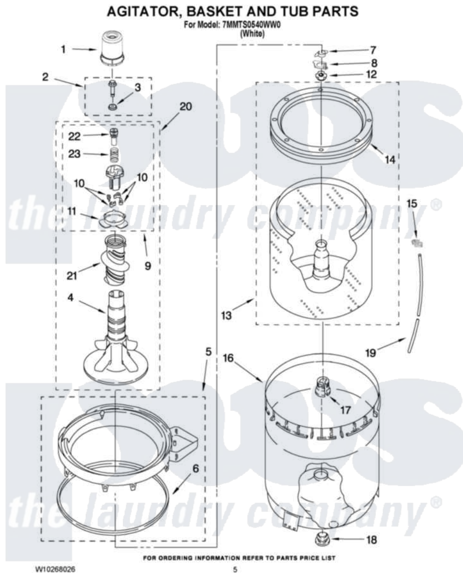
Maytag Residential Maytag 7MMTS0540WW0 Washer Parts Parts Diagram 03 - AGITATOR, BASKET AND TUB PARTS
