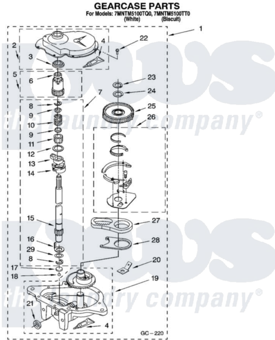
Maytag Residential Maytag 7MNTM5100TQ0 Washer Parts Parts Diagram 08 - GEARCASE PARTS, OPTIONAL PARTS (NOT INCLUDED)
