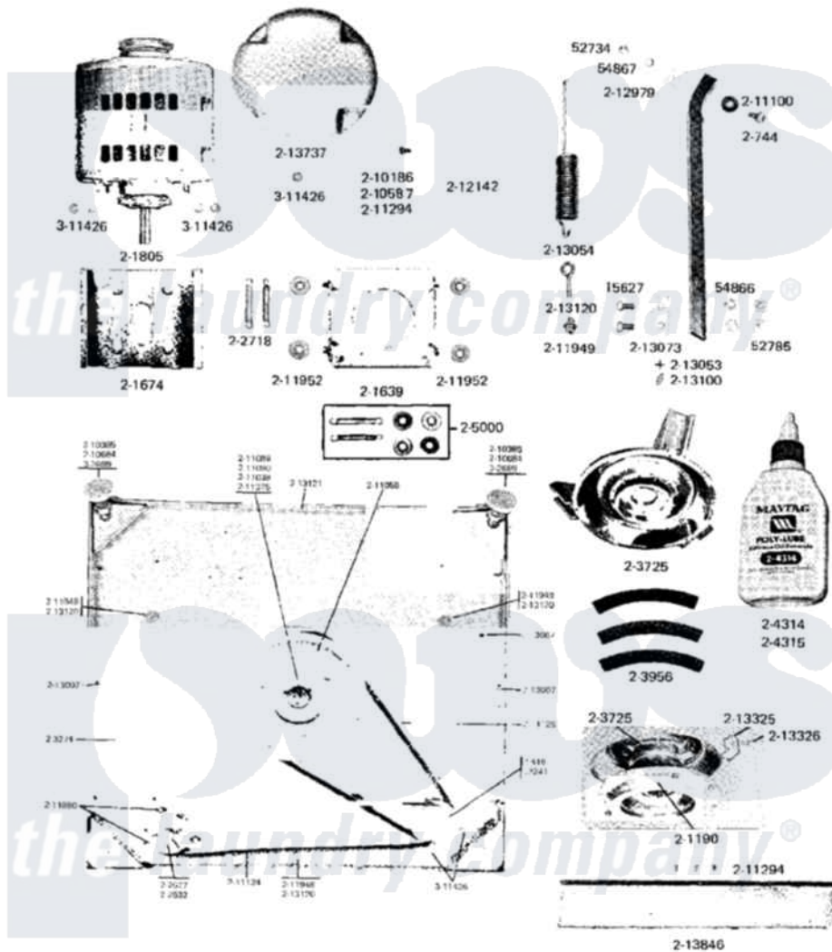
Maytag Residential Maytag A15CM Washer Parts Parts Diagram 07 - MOTOR MOUNT, BASE FRAME & CENTERING SPRS
