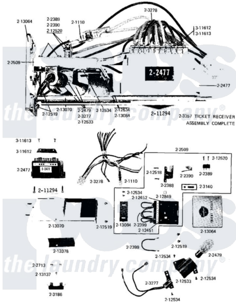
Maytag Residential Maytag A16CT Washer Parts Parts Diagram 03 - CT CONTROL CENTER COMPONENTS Click on the part number to view part
