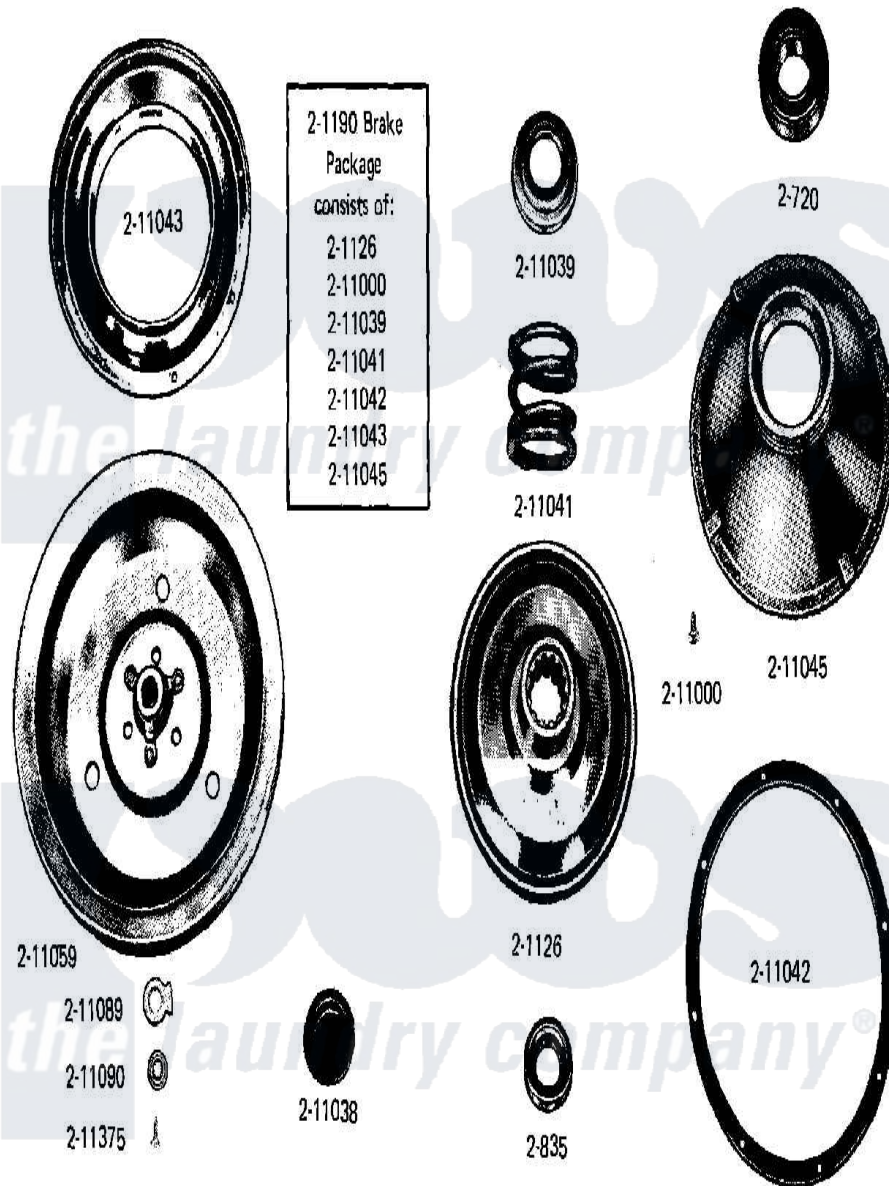
Maytag Residential Maytag A16CT Washer Parts Parts Diagram 09 - BRAKE & CLUTCH ASSEMBLY Click on the part number to view part
