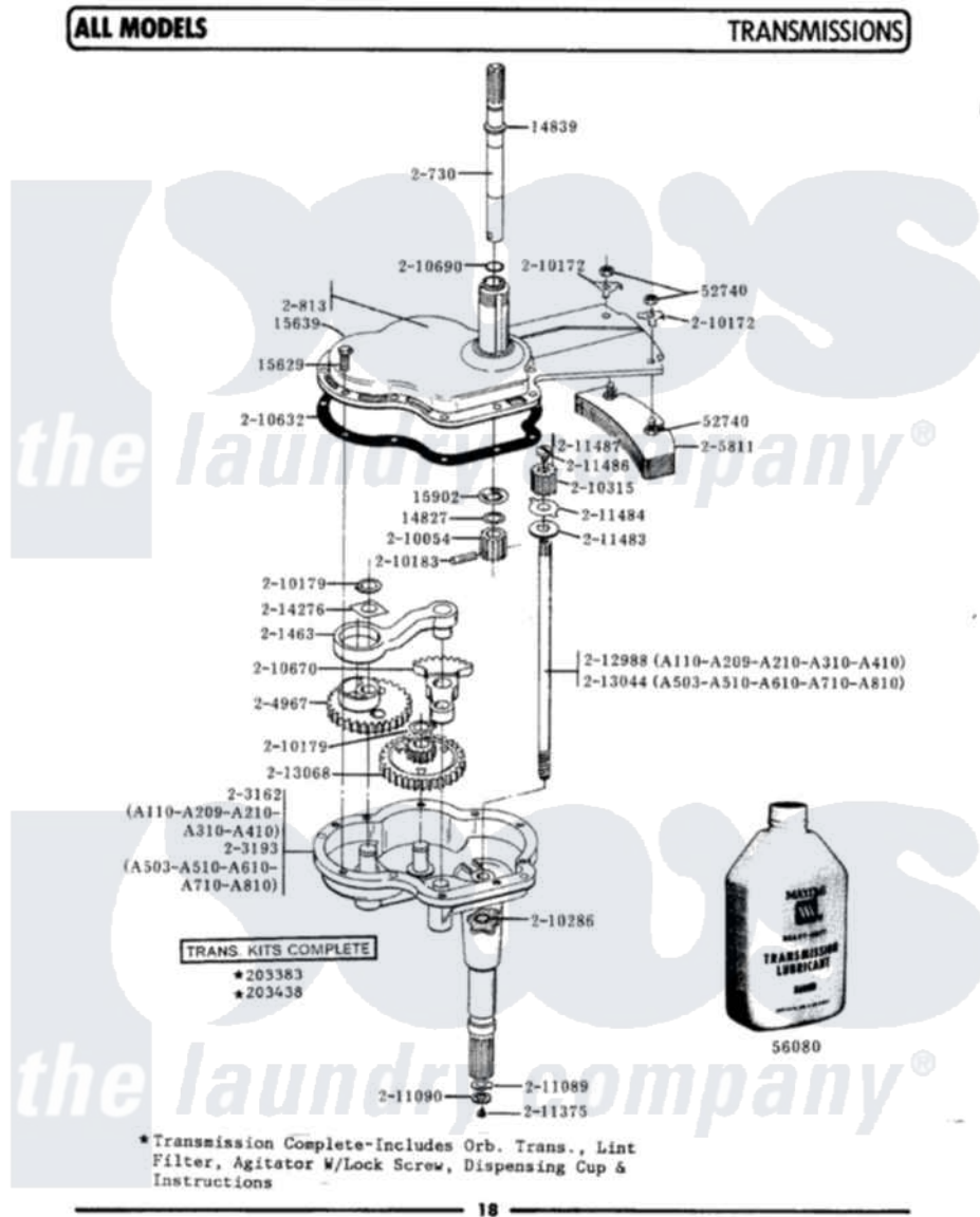
Maytag Residential Maytag A209S Washer Parts Parts Diagram 07 - TRANSMISSIONS Click on the part number to view part
