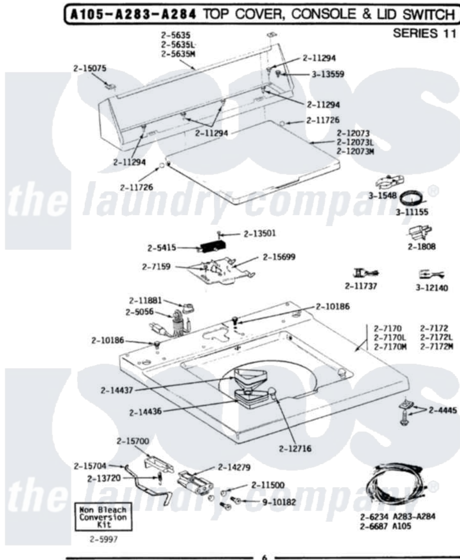
Maytag Residential Maytag A283 Washer Parts Parts Diagram 07 - TOP COVER, CONSOLE & LID SWITCH (SER 11) Click on the part number to view part
