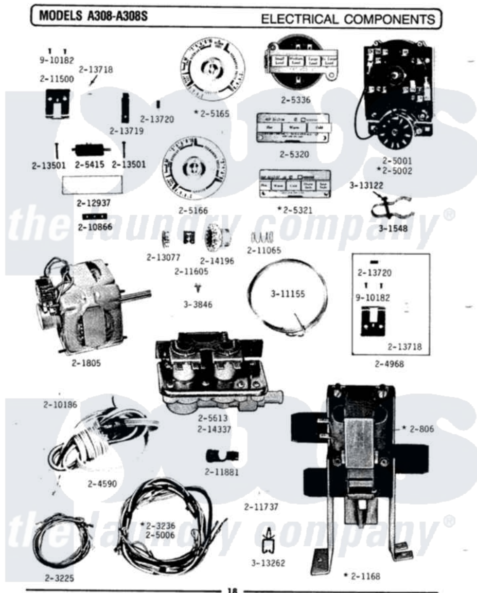
Maytag Residential Maytag A308S Washer Parts Parts Diagram 05 - ELECTRICAL COMPONENTS Click on the part number to view part
