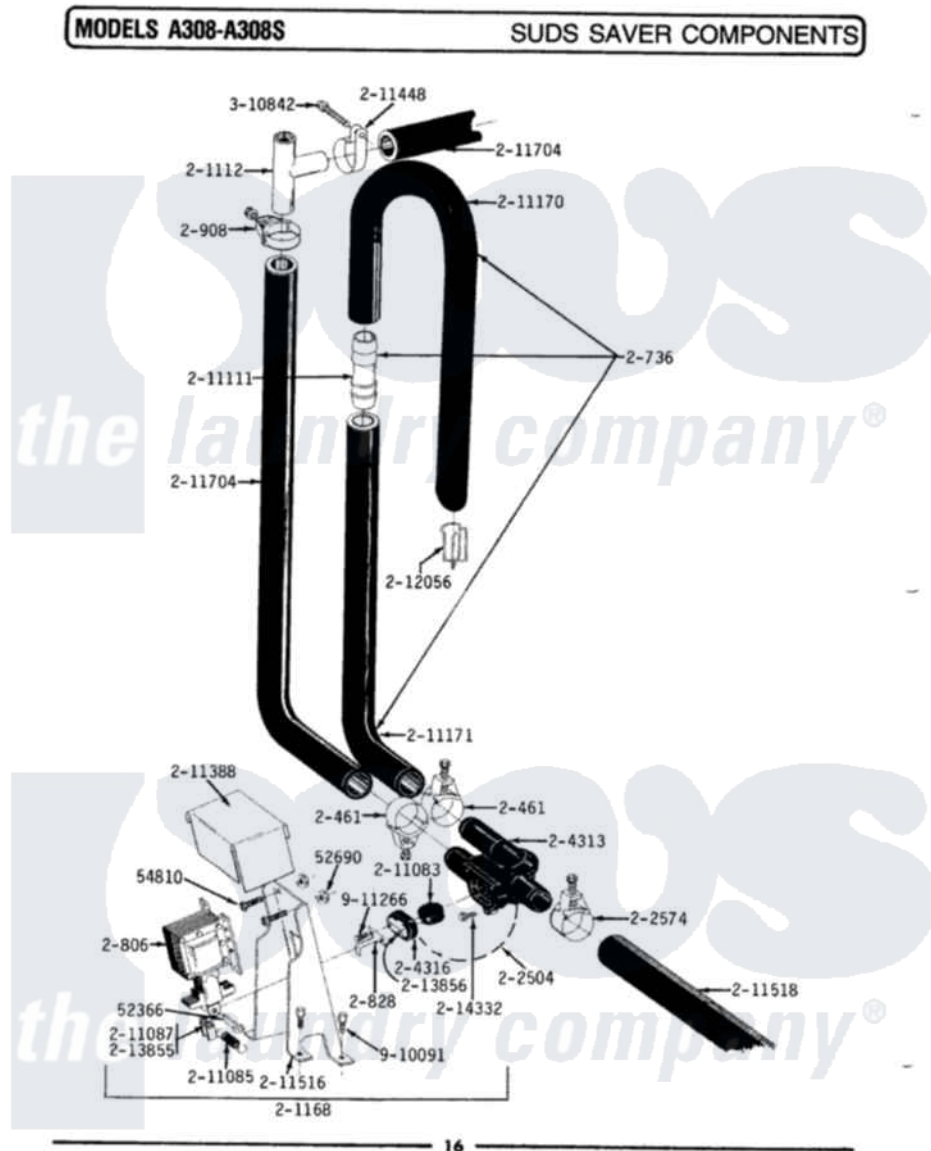
Maytag Residential Maytag A308S Washer Parts Parts Diagram 08 - SUDS SAVER COMPONENTS Click on the part number to view part
