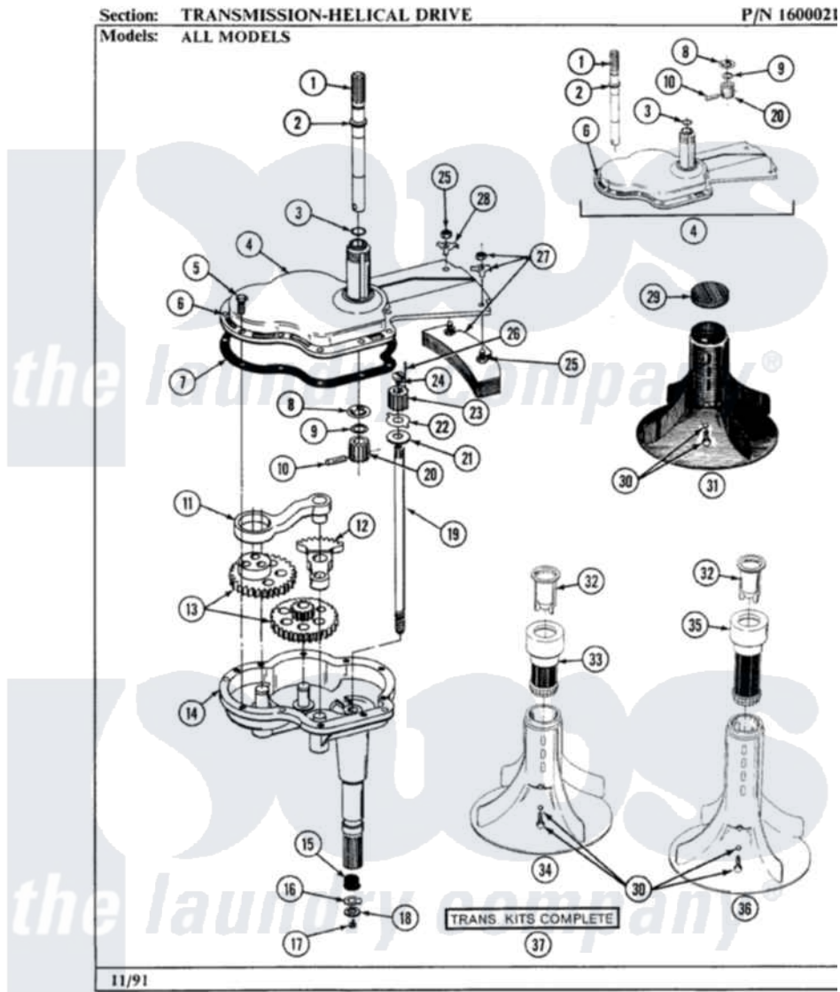
Maytag Residential Maytag A590 Washer Parts Parts Diagram 07 - TRANSMISSION (HELICAL DRIVE) Click on the part number to view part
