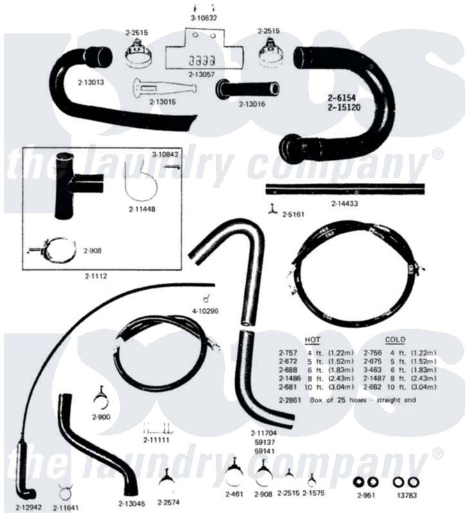
Maytag Residential Maytag A608S Washer Parts Diagram 14 - WATER INJECTION SYSTEM, HOSES & CLAMPS
