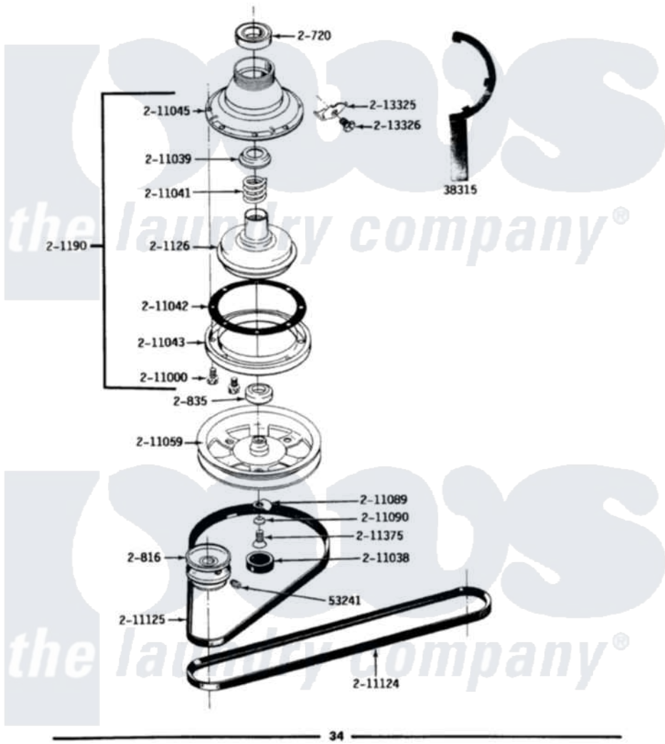
Maytag Residential Maytag A613 Washer Parts Parts Diagram 03 - CLUTCH, BRAKE & BELTS Click on the part number to view part
