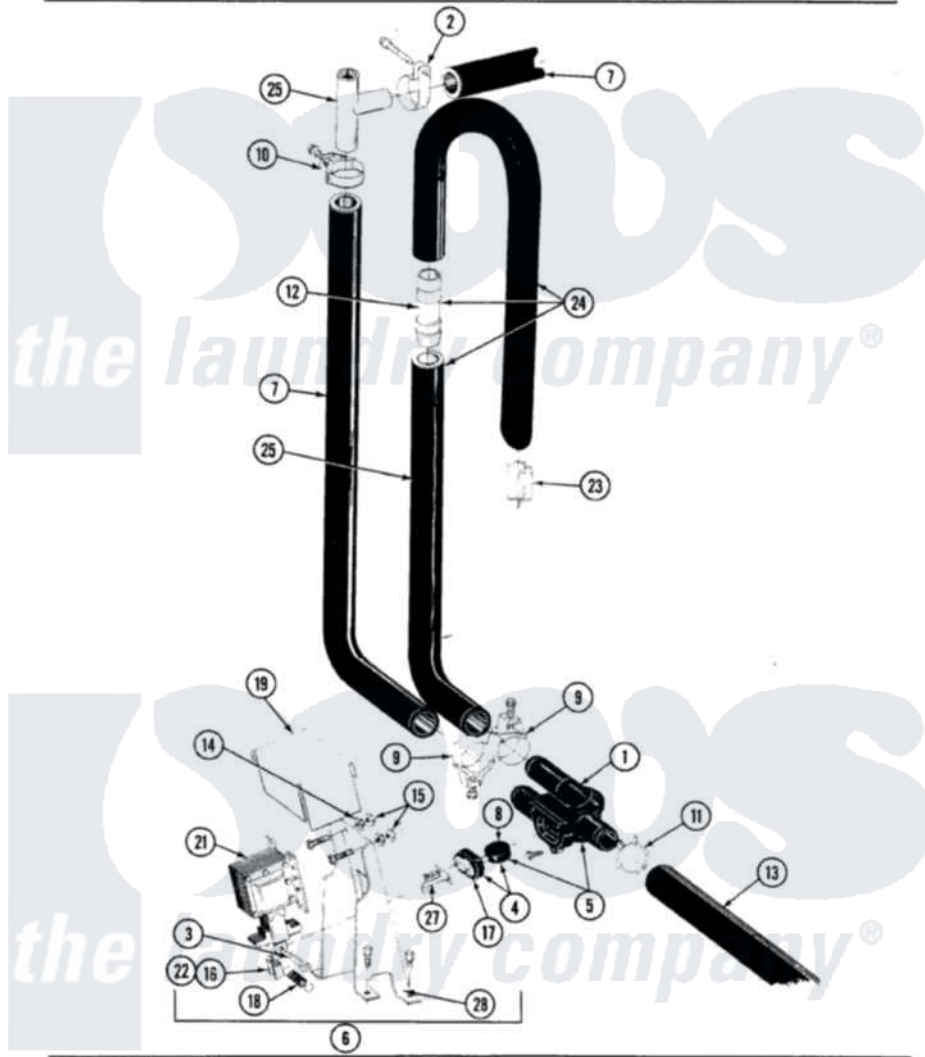
Maytag Residential Maytag A7500S Washer Parts Parts Diagram 08 - WATER SAVER COMPONENTS Click on the part number to view part
