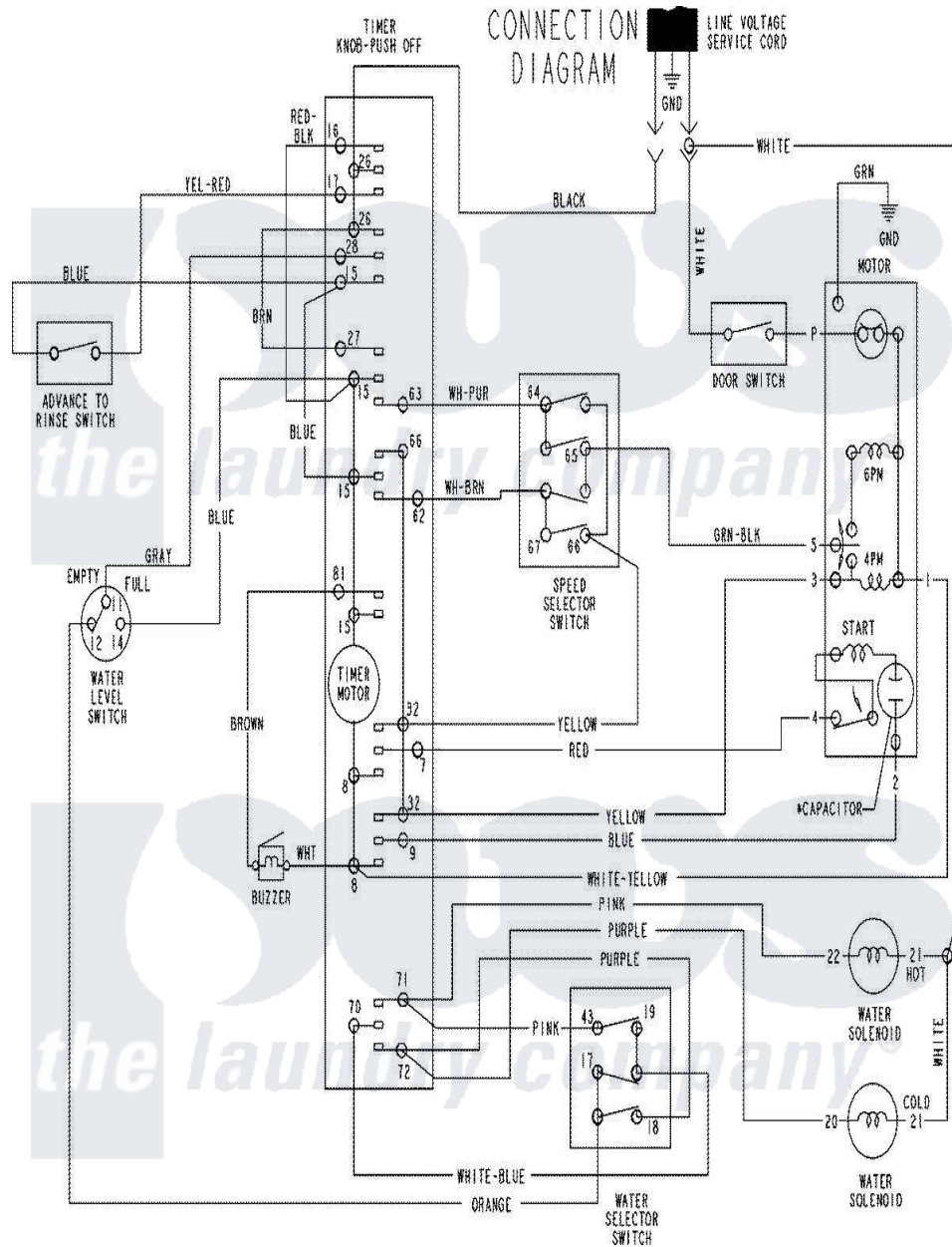
Maytag Residential Maytag AAV8000AJW Washer Parts Parts Diagram 07 - WIRING INFORMATION Click on the part number to view part
