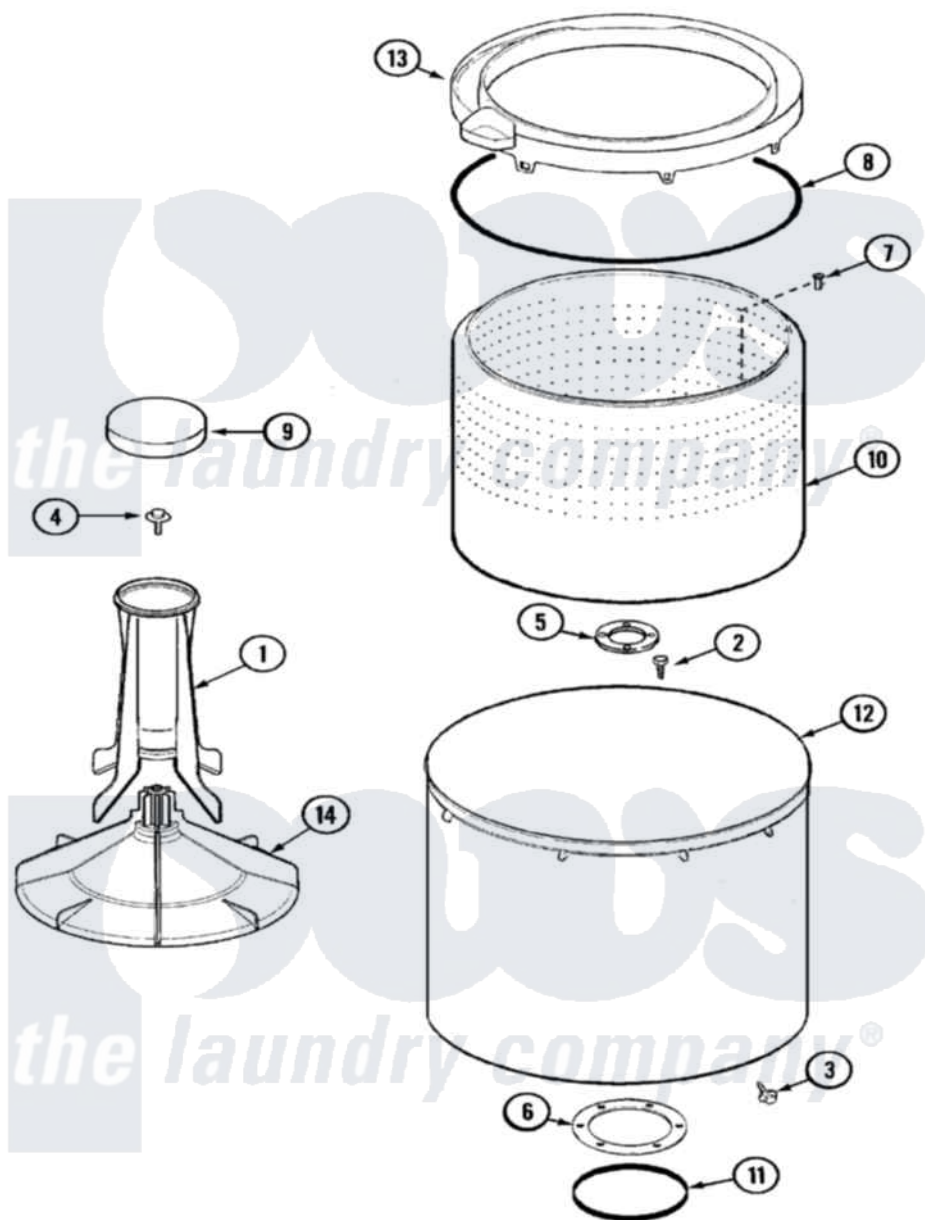
Maytag Residential Maytag CAV2004AKW Washer Parts Parts Diagram 08 - TUB Click on the part number to view part
