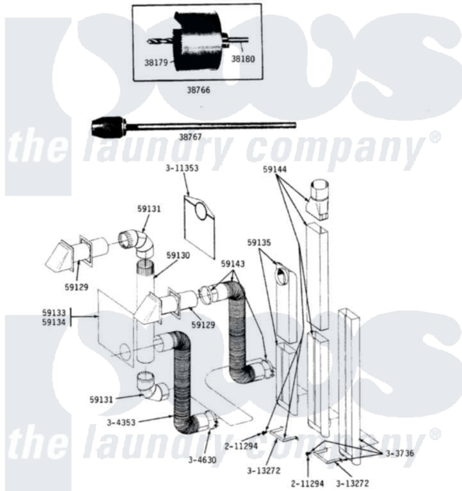
Maytag Residential Maytag DE16CA Dryer Parts Parts Diagram 07 - INSTALLATION ACCESSORIES Click on the part number to view part
